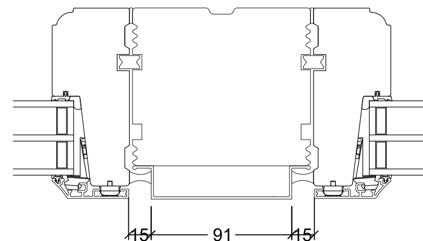
123mm frame Timber: 1033.0174 Aluminium: 52.0049
