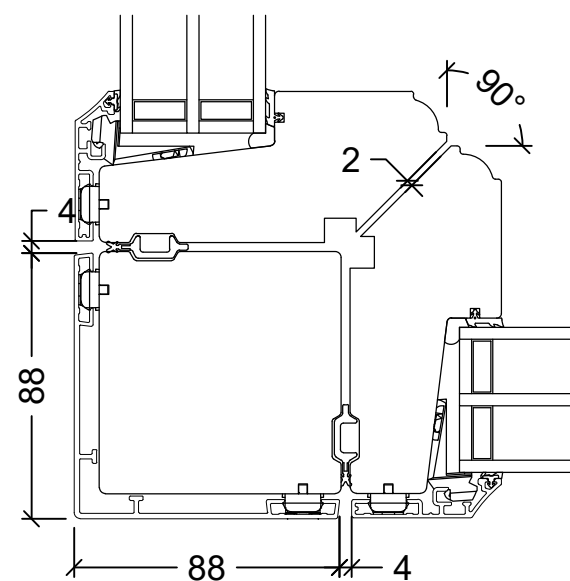
123mm frame Timber: 30.0151 Aluminium: 52.0199 Alignment profile: 50.0245 Bevelling: 45 degree
