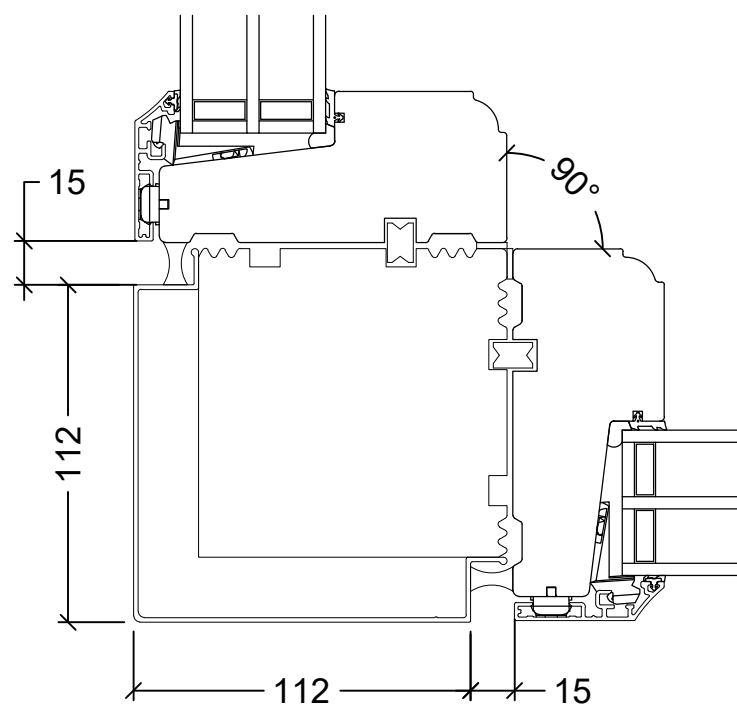
123mm frame Timber: 1033.0169 Aluminium: 52.0048
