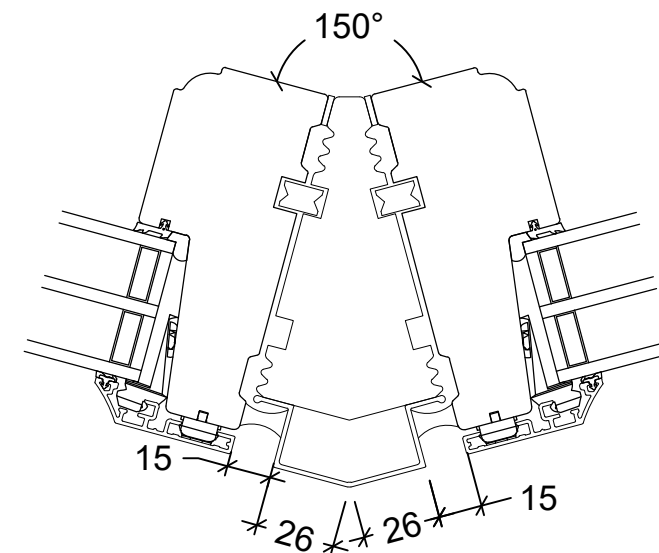
123mm frame Timber: 1033.0166 Aluminium: 52.0002
