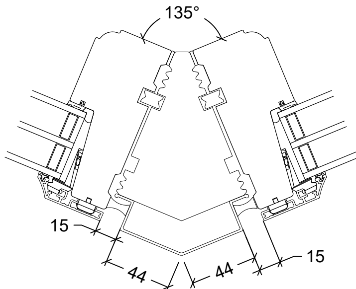
123mm frame Timber: 1033.0167 Aluminium: 52.0003
