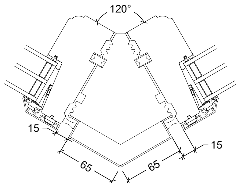
123mm frame Timber: 1033.0168 Aluminium: 52.0004
