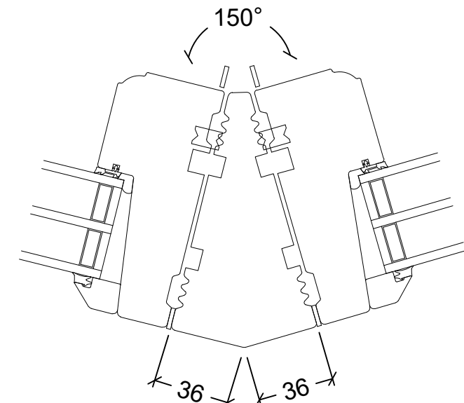
115mm frame Timber: 1033.0170
