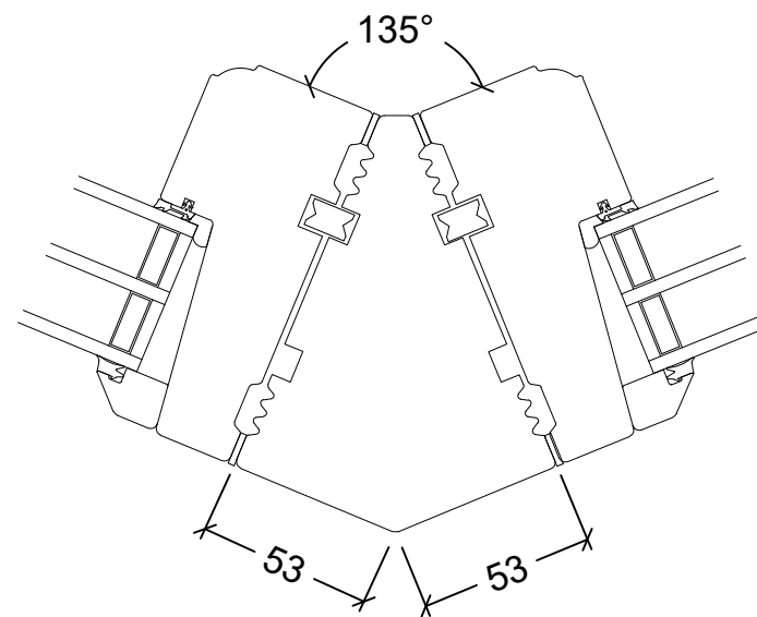
115mm frame Timber: 1033.0171
