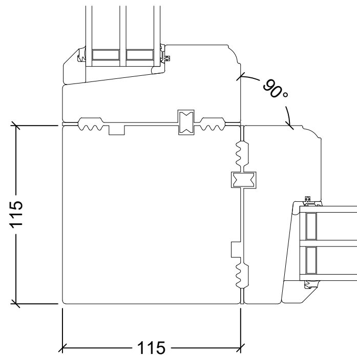
115mm frame Timber: 1033.0173
