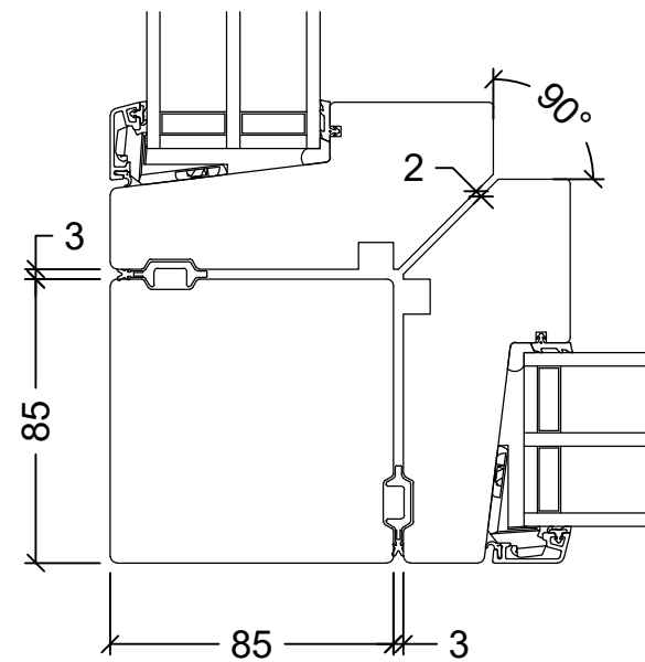
115mm frame Timber: 30.0152 Alignment profile 50.0245 Bevelling: 45 degree
