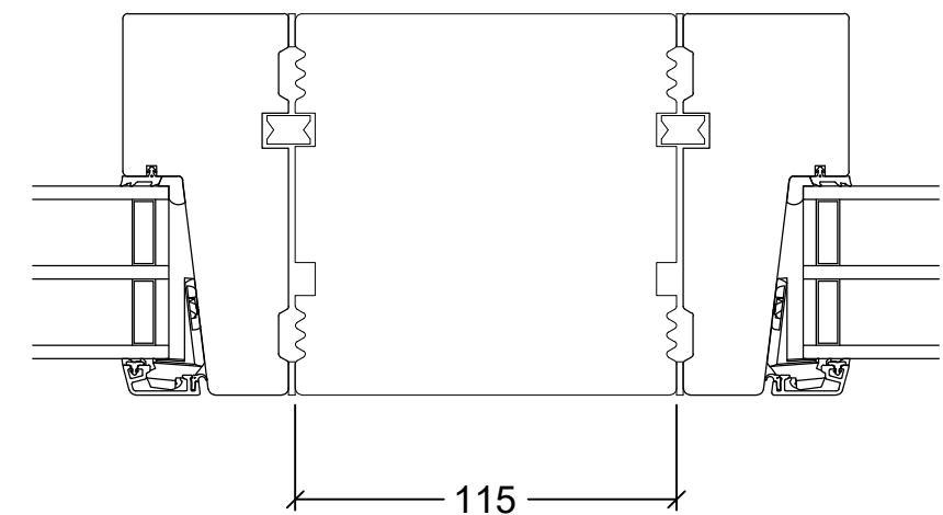
115mm frame Timber: 1033.0175
