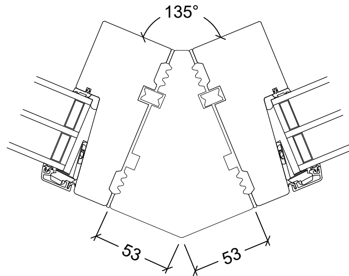
115mm frame Timber: 1033.0171
