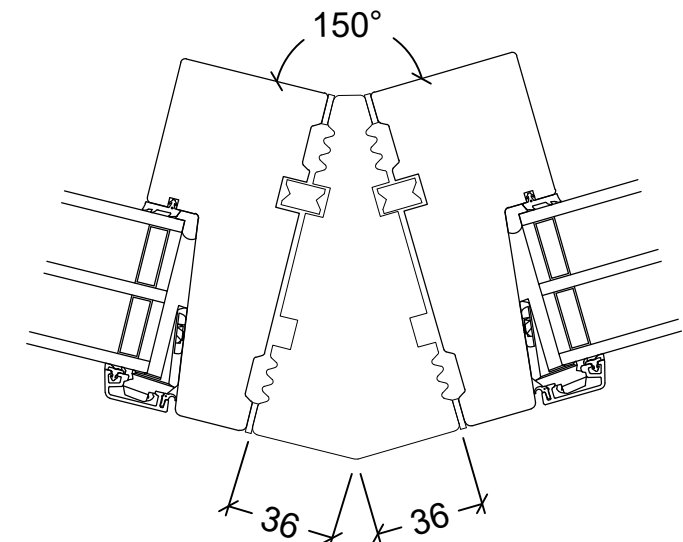
115mm frame Timber: 1033.0170
