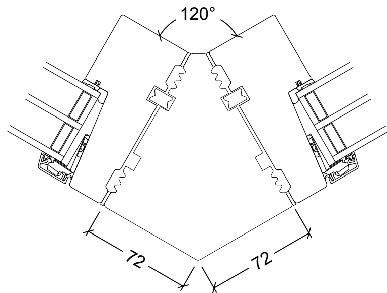
115mm frame Timber: 1033.0172
